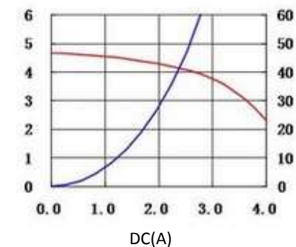
7. CD6020MBDS-150MC
