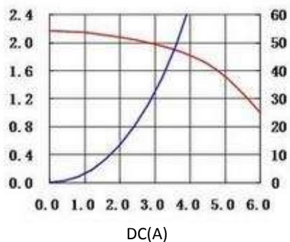
5. CD6020MBDS-6R8MC
